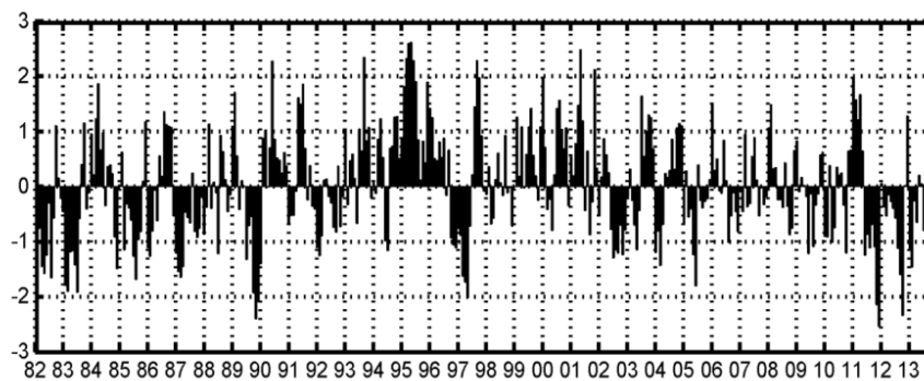
Figure 6.10: Time series of monthly detrended Reynolds SST anomalies f divided by standard deviation in Southern Angola averaged from 10°S to 15°S and from the coast to 1 degree offshore (top) and Northern Namibia averaged from 19°S to 24°S and from the coast to 1 degree offshore( bottom) from 1982 to 2013
