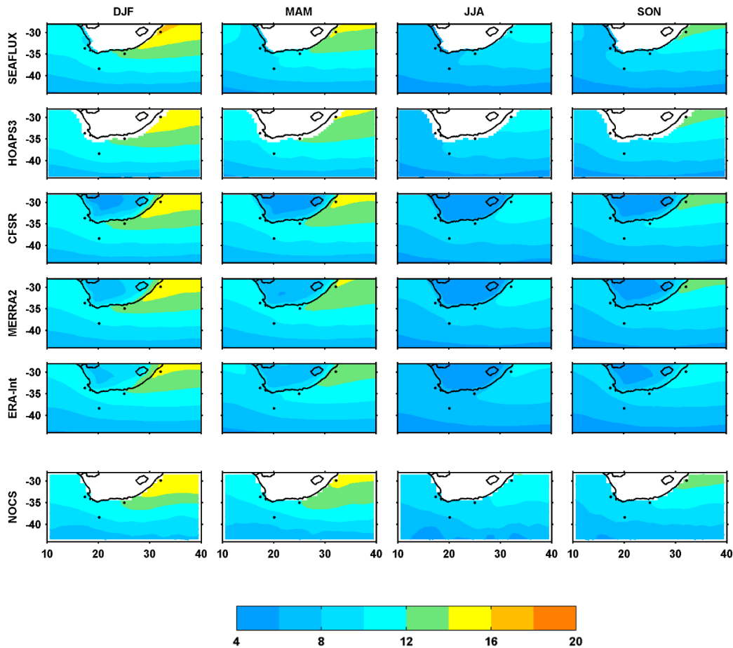
Figure 4.14: From top to bottom: seasonal average of specific humidity of air Q_a (g/kg) of SEAFLEX, HOAPS3, CFSR, MERRA-2, ERA-Interim and NOCS. From left to right Austral summer (DJF), austral fall (MAM), austral winter (JJA) and austral autumn (SON). Black stars represent the fourth locations taken for the study. Agulhas Current off Durban (32°E, 30°S), Agulhas Current off Port Elizabeth (25°E, 35°S), Agulhas Retroflection (20°E, 38.5°S) and Off Cape Town (17°E, 33.7°S).
