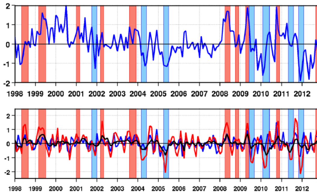
Figure 7.4: Top, Detrended monthly anomalies of zonal wind stress ( N/m^2 ) averaged over ATL4 ( 50^\circ W-25^\circ W, 3^\circ S-3^\circ N ); bottom, OLM detrended anomalies of Kelvin waves monthly contribution to sea level in cm: 1st baroclinic mode in blue line, 2nd baroclinic mode in red line, and 3rd baroclinic mode in black line, averaged over ( 20^\circ W-0^\circ E , at 0^\circ N ). Based on Figure 7.1 (top), abnormal positive and negative propagations of SLA are represented by red and blue rectangles respectively.
