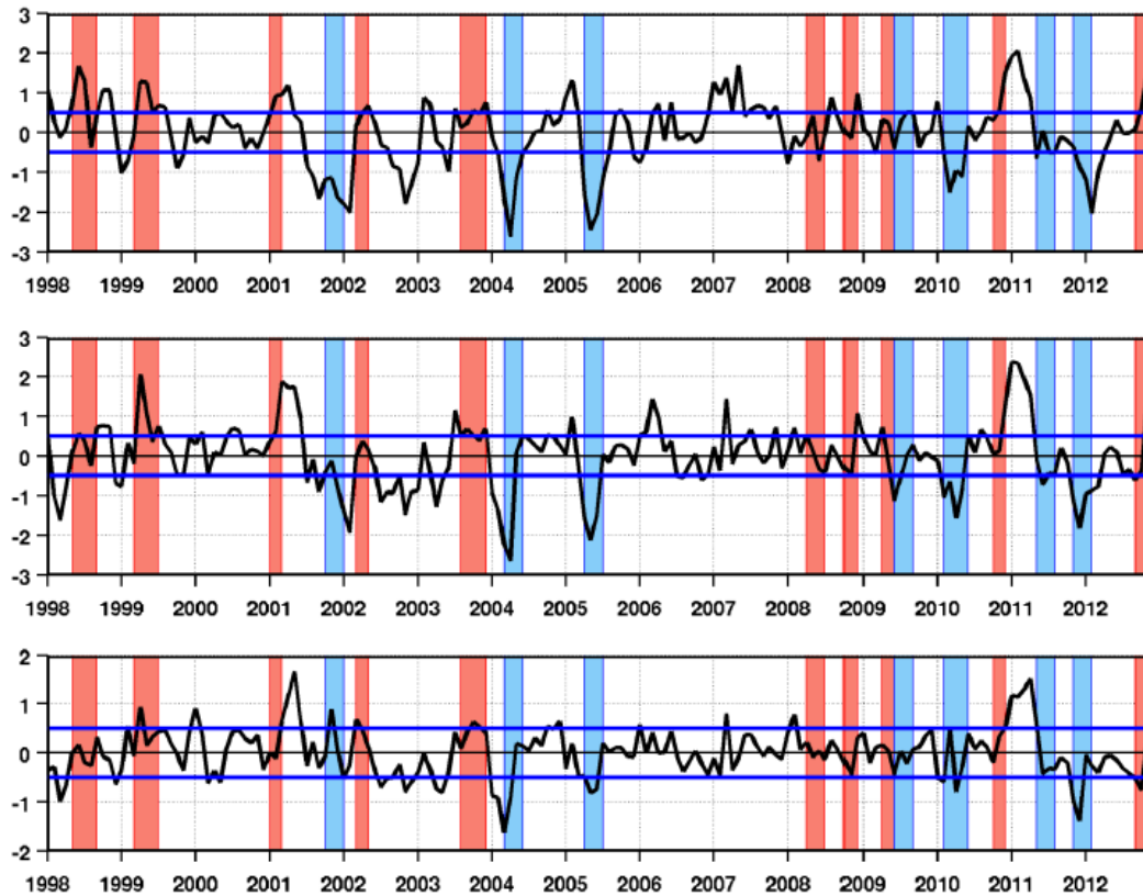
Figure 7.5: Monthly detrended anomalies of SST (°C) in (top) Southern Angola averaged from 10°S to 15°S and from the coast to 1° offshore, (middle) Angola Benguela Front averaged from 16.5°S to 17.5°S and from the coast to 1° offshore and (bottom) Northern Namibia averaged from 19°S to 24°S and from the coast to 1° offshore. The standard deviation is represented by the blue horizontal line. Based on Figure 7.1 (top), abnormal positive and negative propagations of SLA are represented by red and blue rectangles respectively.
