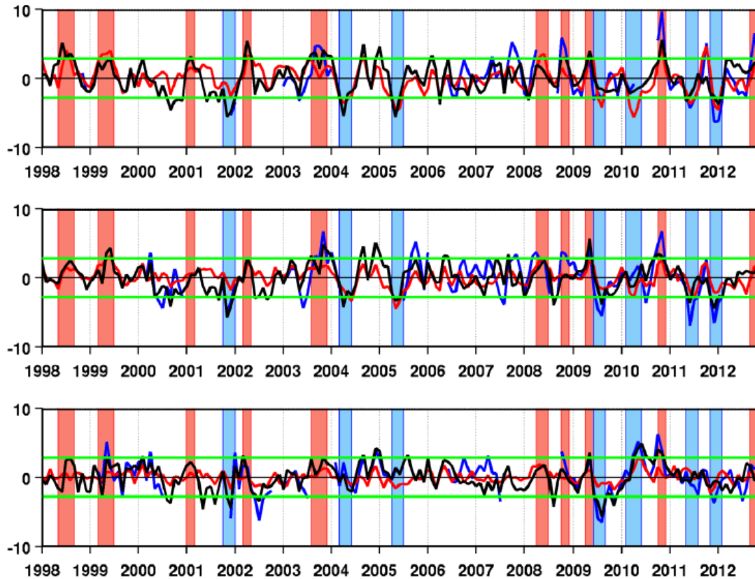
Figure 7.1: Monthly Detrended interannual anomalies of dynamic height (cm) from PIRATA in blue line, Aviso SSH monthly anomaly in black line and SSH monthly anomaly OLM in red line; top, at [0^{\circ}\text{E}, 0^{\circ}\text{N}] ; middle, at [10^{\circ}\text{W}, 0^{\circ}\text{N}] and bottom, at [23^{\circ}\text{W}, 0^{\circ}\text{N}] . The standard deviation derived from PIRATA is represented by the green horizontal line. Based on Figure 7.1 (top), abnormal positive and negative propagations of SLA are represented by red and blue rectangles respectively.
