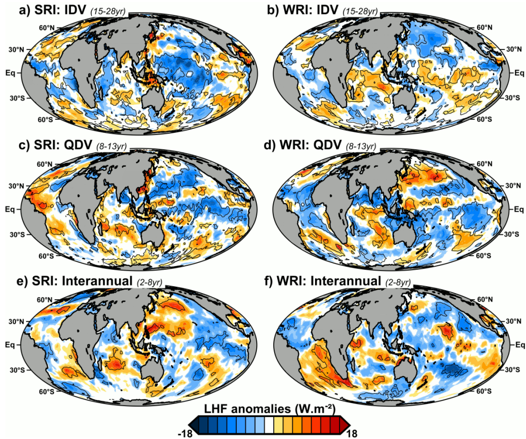
Figure 3.7. as for Figure 3.4, but for latent heat flux (LHF; in \text{W.m}^{-2} ).
