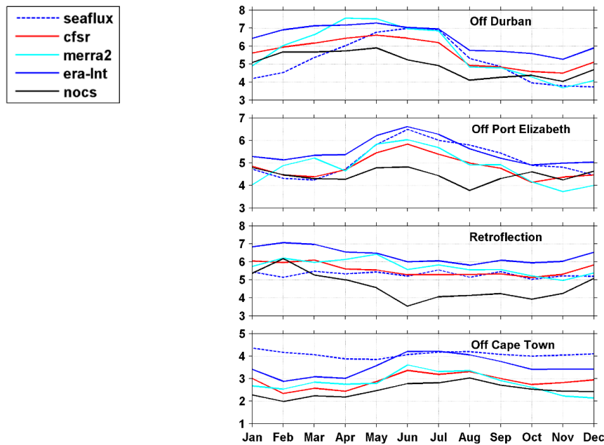
Figure 4.15: Annual cycle of the difference between Qsst and Qa: Off Durban, Off Port Elizabeth, Retroflection and Off Cape Town. For SEAFLUX, CFSR, MERRA-2, ERA-Interim and NOCS.
