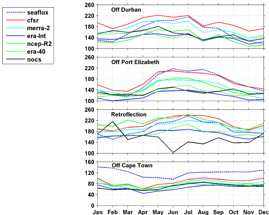
Figure 4.3: annual cycle of latent heat flux ( W/m^2 ). In Agulhas Current off Durban ( 32^\circ E, 30^\circ S ), Agulhas Current off Port Elizabeth ( 25^\circ E, 35^\circ S ), Agulhas Retroflection ( 20.5^\circ E, 38.5^\circ S ) and off Cape Town ( 17^\circ E, 33.7^\circ S ) for SEAFLUX (blue dash), CFSR (red), MERRA-2 (cyan), ERA-Interim (blue), NCEP-R2 (green), ERA-40 (dash green) and NOCS (black). All products are averaged from 1998 to 2005, except ERA-40 averaged from 1995 to 2002.
