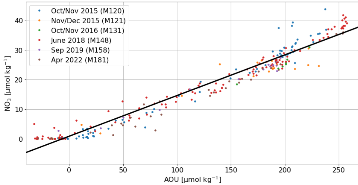
Figure S2: Relationship between Apparent Oxygen Utilization (AOU) and Nitrate (NO 3 ). Dots show the bottle data of CTD casts taken in the upper 400 m. CTD casts were taken during different cruises (colors, see legend). The black line shows the linear fit of the sample data.
