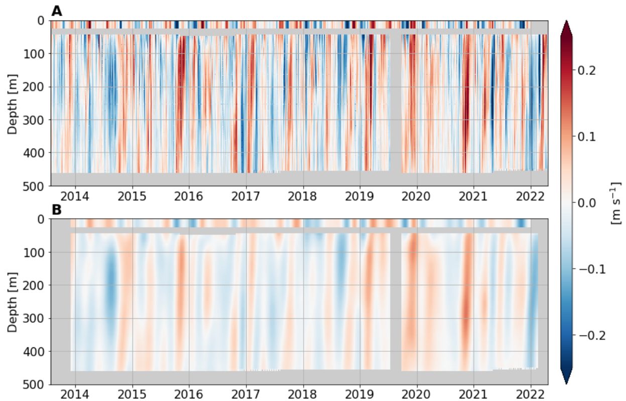
Figure S8: (a) Observed alongshore velocity (rotated by -34^\circ ) of a mooring installed at 13^\circ 00' \text{E} ; 10^\circ 50' \text{S} (1200 m depth). Positive values represent northward flow and negative velocities southward flow. (b) shows the same as (a), but intraseasonal variability is removed by applying a low-pass filter (cutoff period = 130 days). At the surface, the corresponding geostrophic alongshore velocities from SLA are plotted. The mean velocity profile has been subtracted. The geostrophic velocities are taken from the SLA DUCAS satellite data product ( https://doi.org/10.48670/moi-00148 ).
